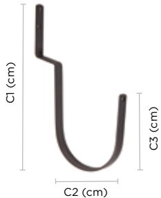
Holdback for Rosette with Separation
